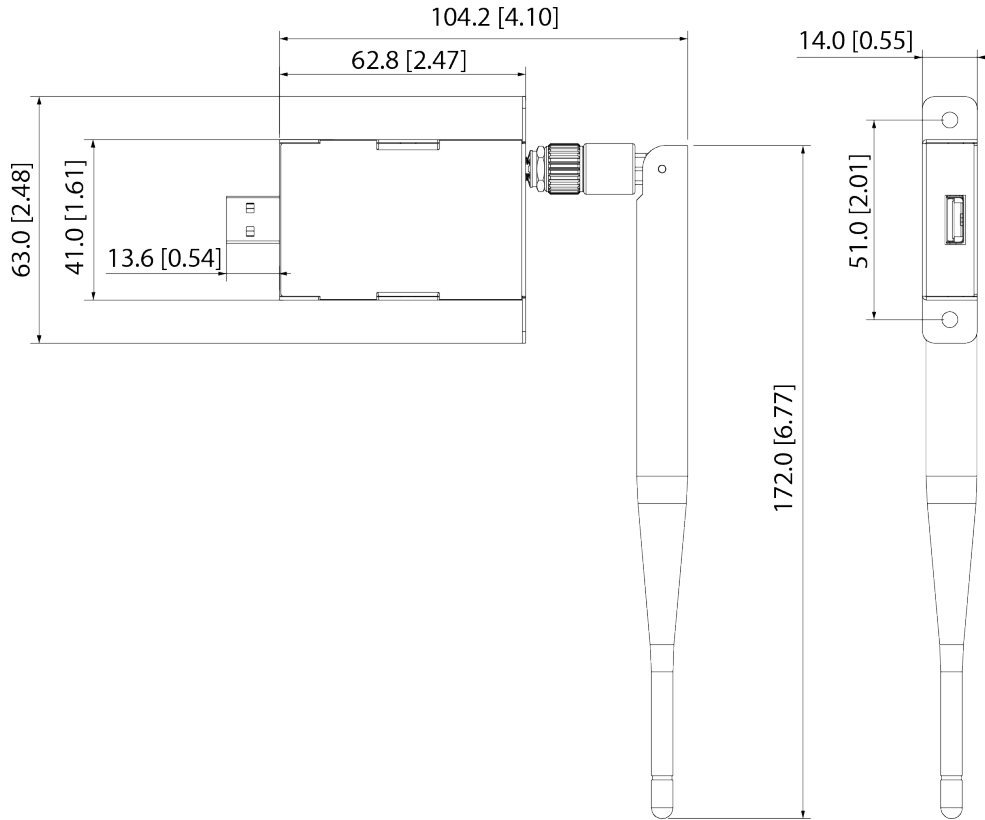
Figure 2-1 Dimensions (mm [inch])
